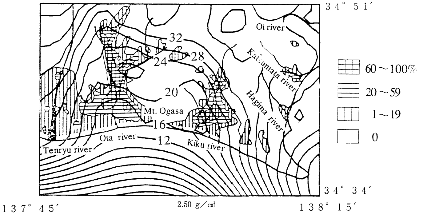
Fig. 3. Bouguer gravity anomaly (density: 2.50 g/cm 3 , contour interval: 2 mGal). Disaster distribution by the 1944 Tonankai earthquake is also shown in this figure.
