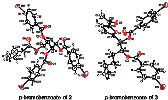
Fig. 3. ORTEP drawings of p -bromobenzoate of 2 and 3 with ellipsoids at the 30% probability level. Hydrogen atoms are shown as small spheres of arbitrary radii.
