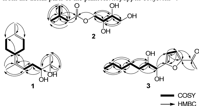
Fig. 2. COSY and HMBC correlations in 1 to 3 .
