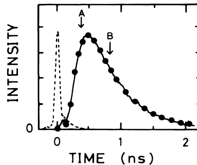
FIG. 1. The solid line is a spatially ensemble-averaged temporal profile of a transmitted 70-ps pulse. Solid circles represent a calculated curve based on the diffusion approximation. The dashed line is the instrument response function to the input pulse. Arrows A and B indicate points of time when the time-resolved memory effect was examined.
