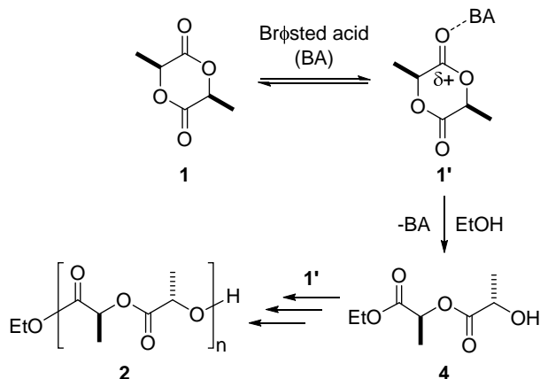
Scheme 5. Proposed mechanism of Brønsted acid-catalyzed ROP in \text{scCO}_2 .
