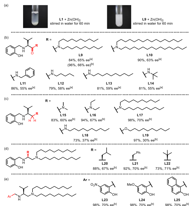
Figure 1. Screening of chiral aminophenols for \text{Zn}(\text{OH})_2 -catalyzed allylation of acetophenone in water. Reactions were carried out with acetophenone (0.200 mmol), 1a (0.300 mmol), \text{Zn}(\text{OH})_2 (10 mol %), and L (11 mol %) in water ([a] 0.04 M or [b] 0.4 M for acetophenone, respectively) for 24 h.
