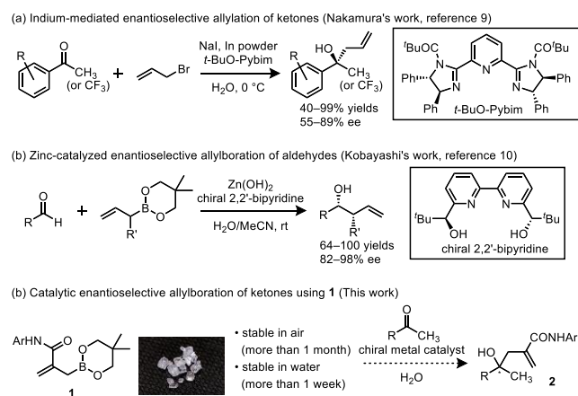
Scheme 1. Enantioselective allylation in aqueous media.
