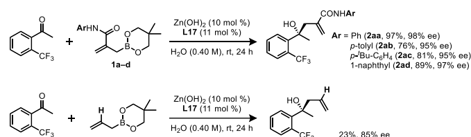
Scheme 3. Effect of amide functionality on 1 .
