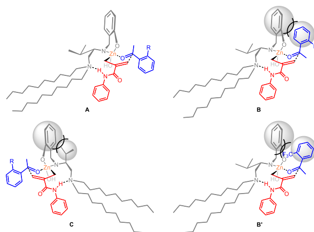
Figure 2. Plausible transition states for enantioselective amido-functionalized allylation in water.
