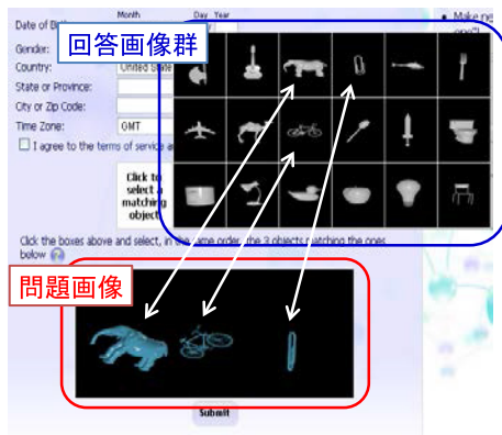
図 3 YUNiTi CAPTCHA
