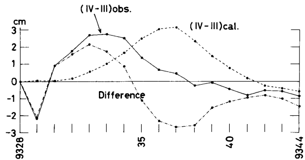
Fig. 3. Estimated vertical movement accompanied by the Kita-Izu earthquake of 1930, "Difference". (IV - III) obs. is the survey result for IV and III, and (IV - III) cal. is movement which is extrapolated from the mean speed of movement in I (since Feb., 1930) ~ II ~ III.
