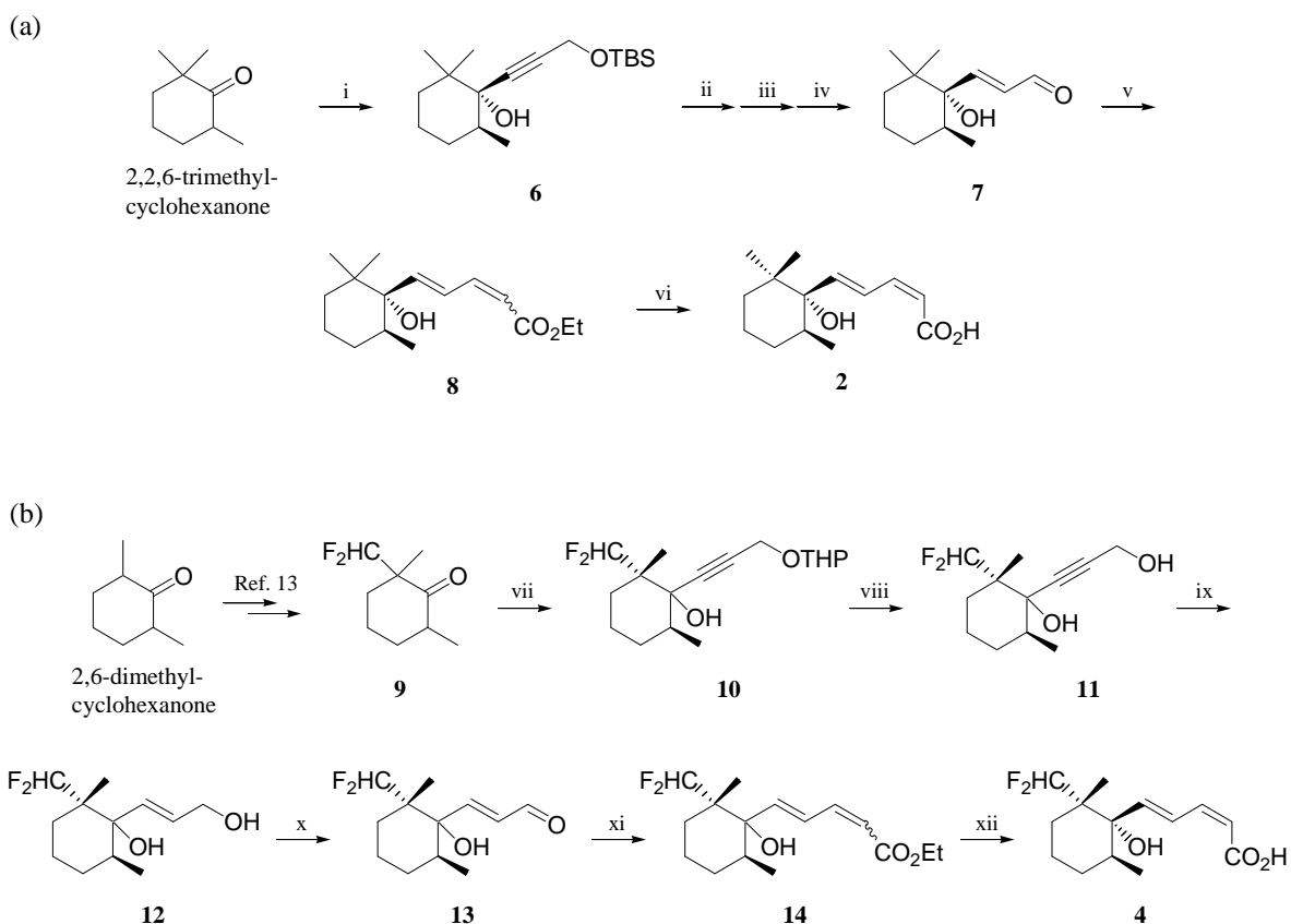
Scheme 1. Synthetic routes of compound 2 (a) and compound 4 (b). Reagents: (i) 2-propynyl TBS ether (3.1 equiv), n -BuLi (2.0 equiv), dry THF, -78\text{ }^{\circ}\text{C} , 50 min, and then addition of 2,2,6-trimethylcyclohexanone, -78 to -11\text{ }^{\circ}\text{C} , 2.5 h, 87%; (ii) SMEAH (2.9 equiv), dry THF, RT, 1.5 h; (iii) THF:AcOH:H 2 O = 1.5:3:1 (v/v), RT, 3 d, 71% from 6 ; (iv) PDC (1.3 equiv), Celite, dry CH 2 Cl 2 , RT, 4 h, 85%; (v) ethyl di- o -tolylphosphonoacetate (3.3 equiv), NaH (4.6 equiv), dry THF, 0\text{ }^{\circ}\text{C} , 30 min, then addition of 7 at -78\text{ }^{\circ}\text{C} , -78 to -24\text{ }^{\circ}\text{C} , 70 min, 87%; (vi) NaOH, MeOH, RT, 4 h, and purification with Sep-Pak Plus C18 cartridges, 63%; (vii) 2-propynyl THP ether (2.7 equiv), n -BuLi (2.1 equiv), dry THF, -75\text{ }^{\circ}\text{C} , 1 h, and then addition of 9 , -30 to -15\text{ }^{\circ}\text{C} , 2.5 h, 46%; (viii) pyridinium p -toluenesulfonate (0.1 equiv), EtOH, 55\text{ }^{\circ}\text{C} , 3.5 h, 83%; (ix) SMEAH (10.5 equiv), dry THF, RT, 1.5 h, 85%; (x) MnO 2 (19.3 equiv), CH 2 Cl 2 , RT, 2.5 h, 74%; (xi) ethyl di- o -tolylphosphonoacetate (1.7 equiv), NaH (3.0 equiv), dry THF, 0\text{ }^{\circ}\text{C} , 30 min, then addition of
