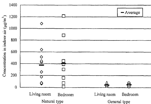
Fig. 9. Limonene air concentration in measured rooms. Notes: Measured rooms are the same as shown in fig. 2.
