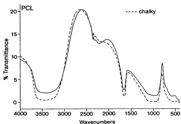
Fig. 3 FT spectra for clear (solid line) and chalky (dotted line) gismondine.
