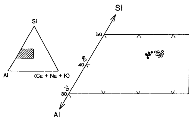
Fig. 4 Compositions of gismondines from Aranga summarised on ternary diagram. Open circles and closed circles represent clear and chalky varieties respectively.
