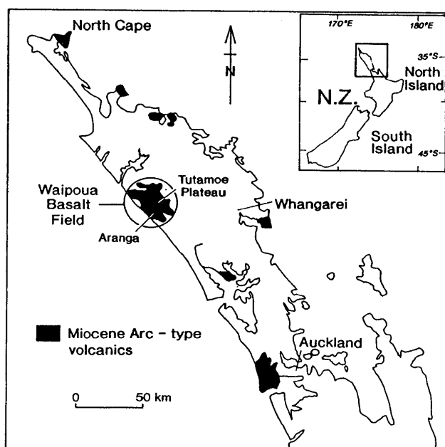
Fig. 1 Locality map for the Waipoua Basalts and Aranga area.
