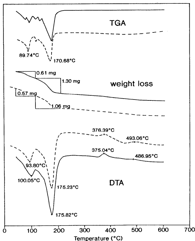
Fig. 5 Thermal data for clear (solid line) and chalky (dotted line) gismondine.
