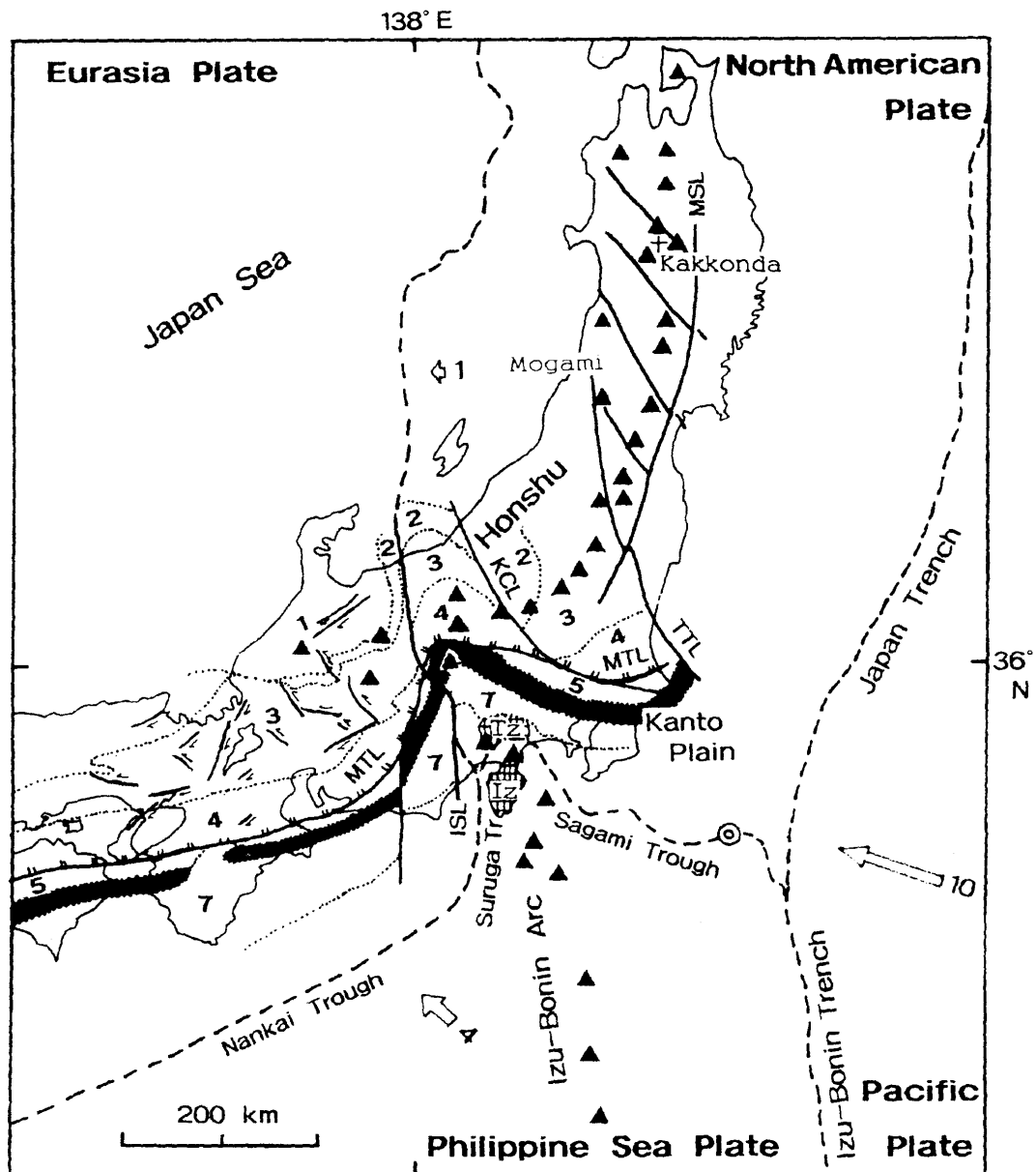
Fig. 1 Plate Tectonic framework of the triple junction and the Philippine Sea Plate. Double circle: trench-trench-trench type triple junction, white arrows: present plate motions in cm/year relative to the Eurasian Plate, arrow length represents the motion for 1 m.y., black triangles: active volcanoes, dotted lines: boundaries of accretionary belts, solid lines: faults, thin arrows: strike slip motion of active faults (Research Group for active faults of Japan, 1994), MTL: Median Tectonic Line (with double tick marks), ISL: Itoigawa-Shizuoka Tectonic Line, KCL: Kashiwazaki-Choshi Tectonic Line, TTL: Tanakura Tectonic Line, MSL: Morioka-Shirakawa Tectonic Line, Tz: Tanzawa Block, Iz: Izu Block, 1: Hida Belt, 2: Hida Marginal-Joetsu Belt, 3: Mino-Tamba-Ashio Belt, 4: Ryoike Belt, 5: Sambagawa Belt, 6: Chichibu and Sambosan Belt (black), and 7: Shimanto Belt.
