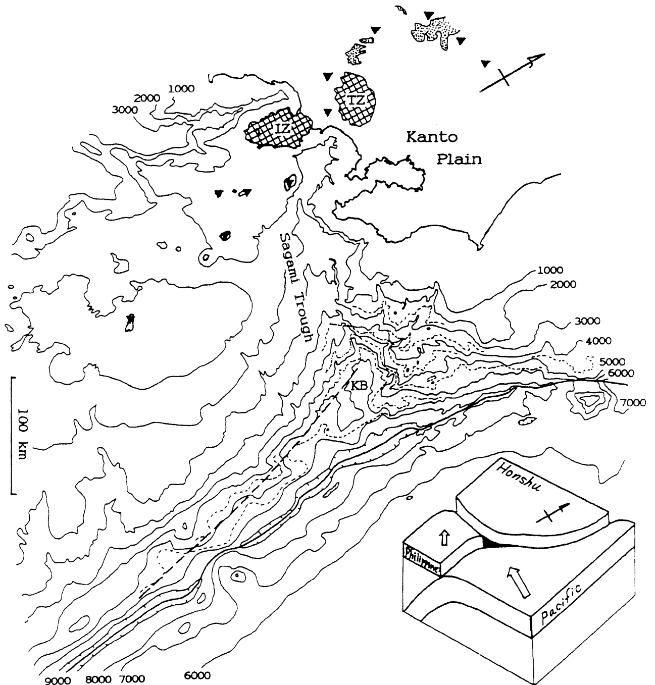
Fig. 3 Collapse topography around the triple junction (Hydrographic Department of Japan, 1991), and block diagram of subducting plates and triangular hole at the triple junction. Depth contours: in meters, solid line: trace of the deepest part along the Japan Trench and Izu-Bonin Trench, broken line: western margin of collapse topography, triangles: active volcanoes, dotted area: late Miocene to Pleistocene volcanics (Geological Survey of Japan 1992), TZ: Tanzawa Block, IZ: Izu Block, KB: Katsura Basin, and white arrows: plate motions.
