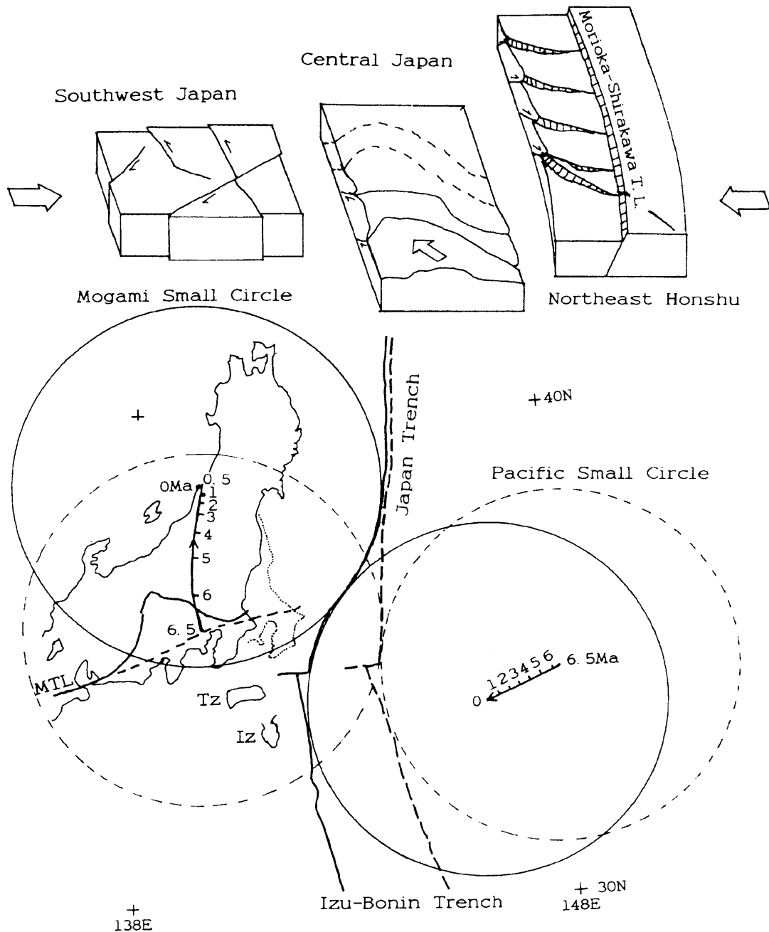
Fig. 4 The Pacific and Mogami Small Circles of present and 6.5 Ma with traces of the center, and tectonic feature of southwest Japan, central Japan and northeast Honshu. Solid line: present plate boundary and MTL (Median Tectonic Line), broken line: plate boundary and MTL at 6.5 Ma, dotted line: position of present coast at 6.5 Ma, Tz and Iz: position of Tanzawa Block and Izu Block at 6.5 Ma.
