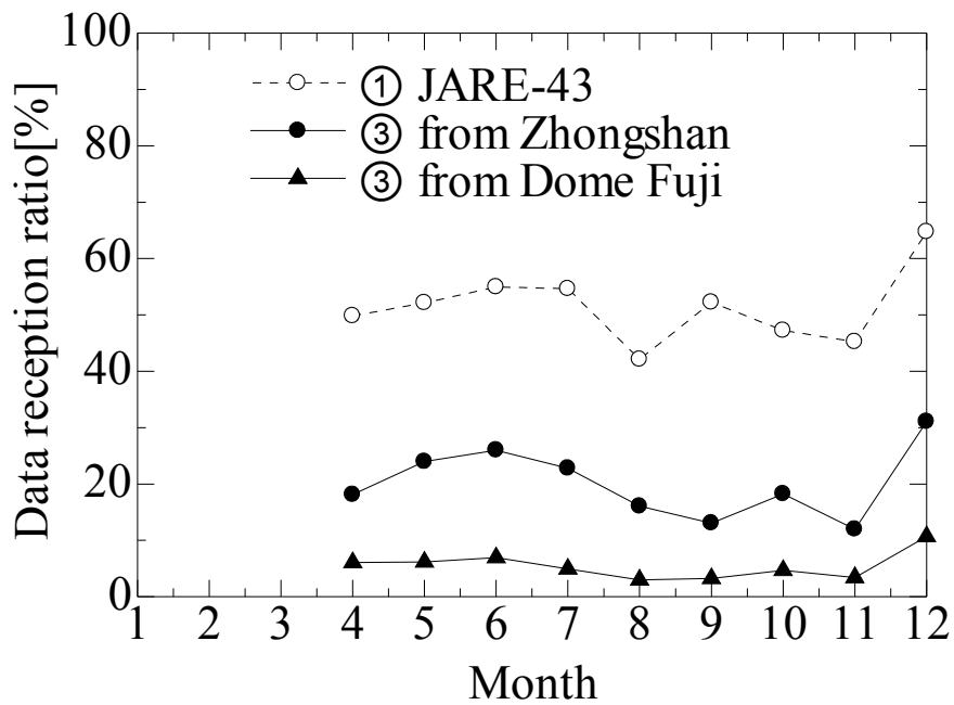
Fig.10 Seasonal variation of data reception ratios (averaged over 00-16UT).
