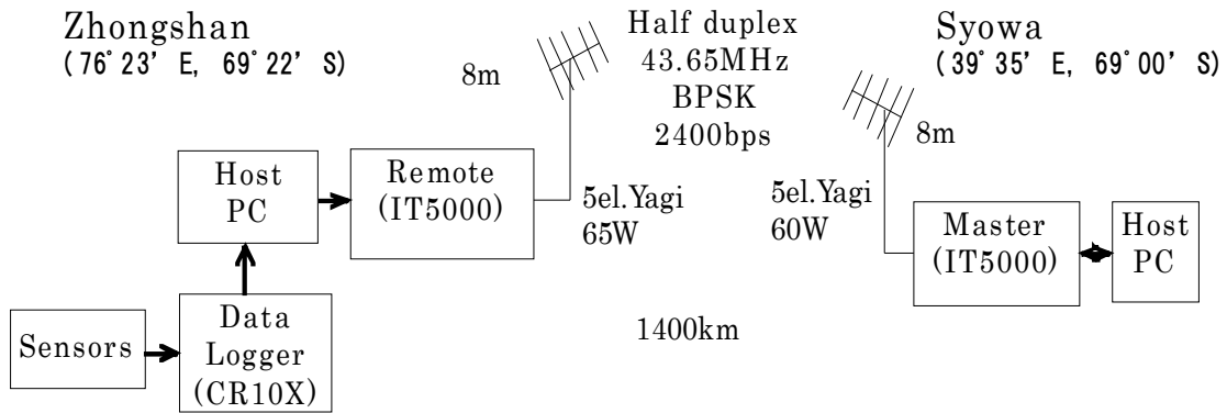
Fig.13. Equipment for the data experiment during the period of JARE-45.
