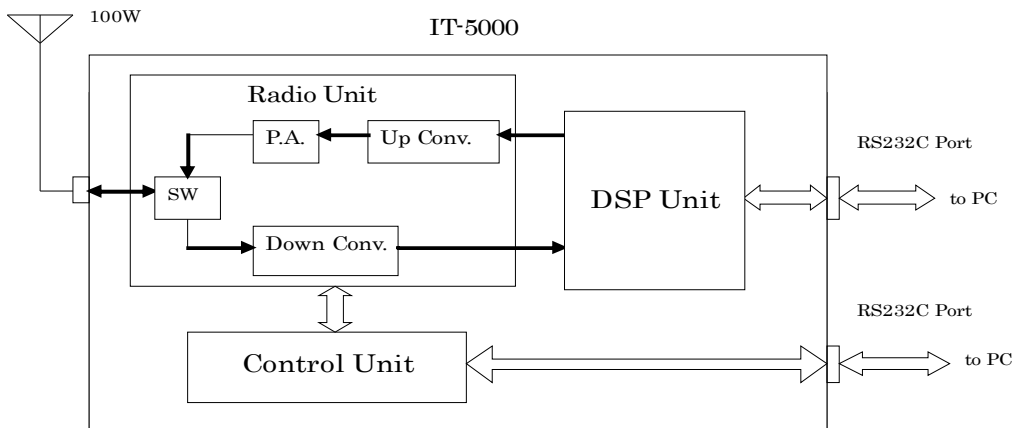
Fig.14 Block diagram of IT-5000.
