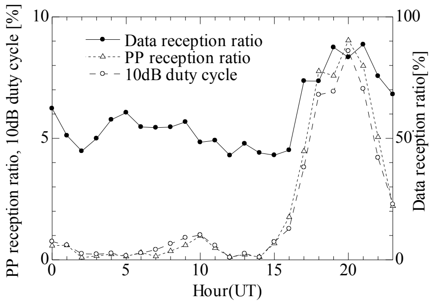
Fig.4. Hourly variations of data reception ratio, PP reception ratio and 10dB duty cycle (Apr.1st-Dec.31st 2002).
