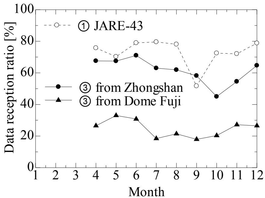
Fig.11. Seasonal variation of data reception ratios (averaged over 16-24UT).
