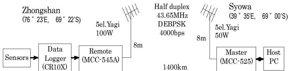
Fig.2. Equipment for the data experiment during the period of JARE-43.
