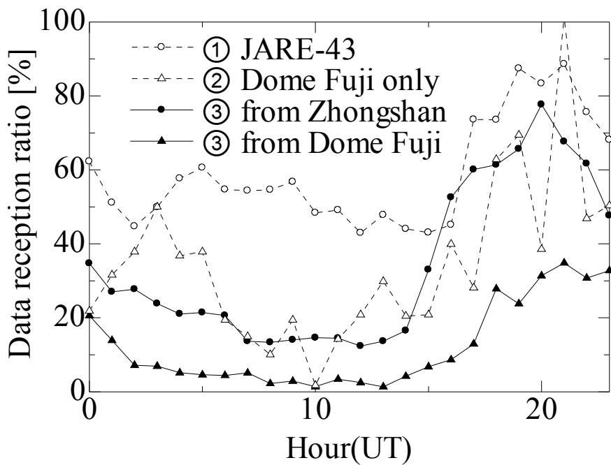
Fig. 8. Hourly variations of data reception ratios (①:Apr.1st-Dec.31st 2002, ②:Feb.27th-Mar.23rd 2003, ③:Mar.25th-Dec.31st 2003).
