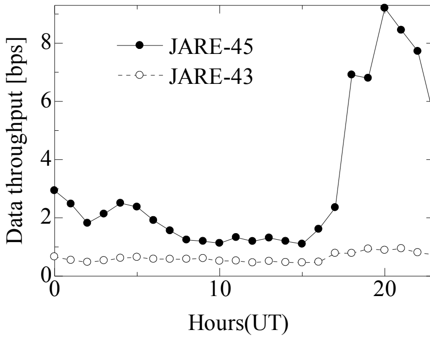
Fig.16. Hourly data throughputs (Apr.1st-Aug.31st 2004 for the experiment in JARE-45, Apr.1st-Dec.31st 2002 for the experiment in JARE-43).
