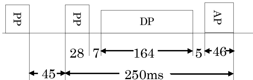
Fig.3. The length and transmission timing of packets used in the data experiment during the period of JARE-43.
