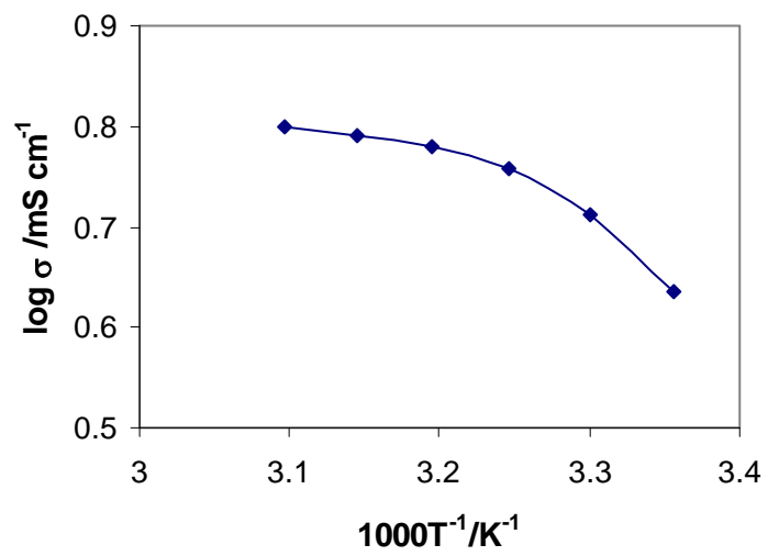
Figure 2. Variation of ionic conductivity with temperature for the PAN electrolyte for composition f having the highest ionic conductivity
