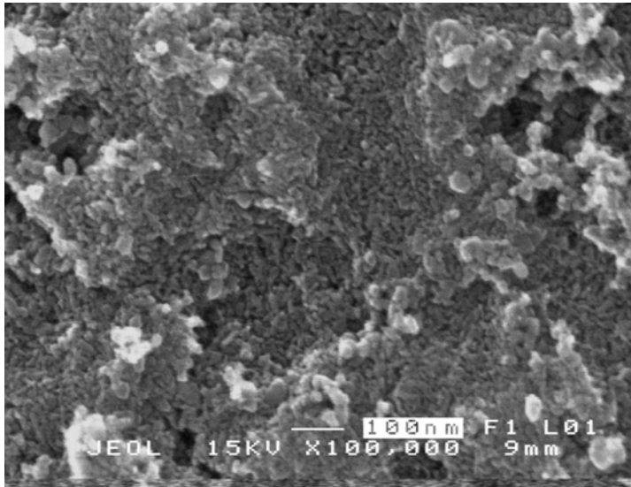
Figure . 1. SEM photographs of the TiO 2 films (a) Film prepared by mixing 0.2 g and 20 ml of colloidal suspension containing 6 nm particles (TiO 2 content 2.2 %, w/w)
