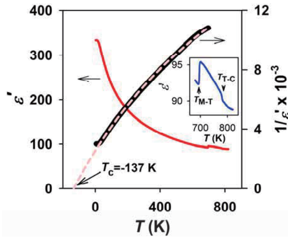
Fig. 26. Temperature dependences of \varepsilon' and 1/\varepsilon' fitted to the modified Curie-Weiss law \varepsilon = \varepsilon_1 + C/(T - T_0) (dashed line, \varepsilon_1 = 38.2 , C = 4.7 \cdot 10^4 K, T_0 = -137 K) for \text{AgTaO}_3 measured at 1 MHz upon heating. The inset further shows the step-like phase transitions from monoclinic to tetragonal and then to cubic at T_{M-T} = 694 K and T_{T-C} = 780 K, respectively.
