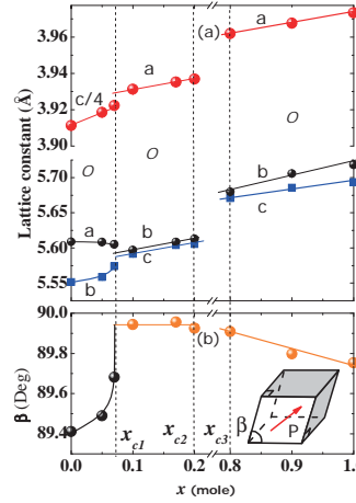
Fig. 18. Lattice parameters change with composition in \text{Ag}_{1-x}\text{K}_x\text{NbO}_3 solid solution. is the orthorhombic distortion angle. The inset shows the orthorhombic distortion due to the ferroelectric displacements along the \langle 110 \rangle_p direction of the pseudocubic structure.
