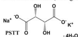
Fig. 1 Molecular structures of buffers used. It is divided into four groups: a , piperazine/morpholine ring with an N-substituted alkyl sulfonate, b N-substituted alkyl sulfonate, c alkyl alkanol amine, and d miscellaneous (inorganic buffer)
