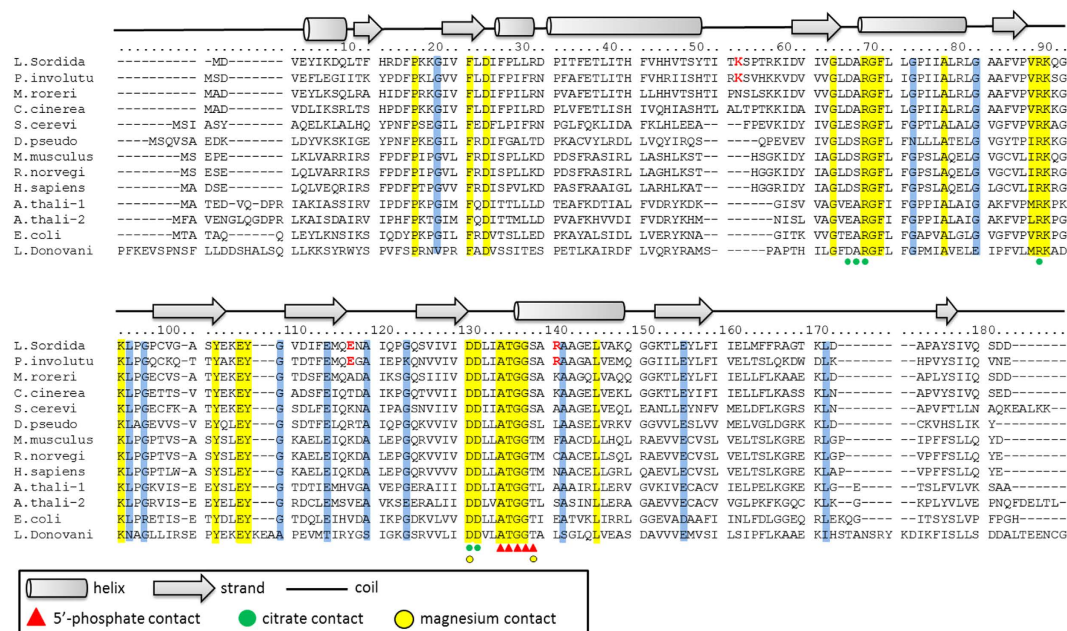
Figure 4. A multiple alignment of APRTs in 13 species. Conserved sequence in all the APRT and 12 APRT are colored in yellow and blue, respectively. Residues involved in 5'-phosphate binding and Mg-pyrophosphate binding were circled in red and in black, respectively. The following APRTs were applied (GenBank accession numbers in parentheses): P. involutu , Paxillus involutus (KIJ20178.1); M. roreri , Moniliophthora roreri (XM_007844891.1); C. cinerea , Coprinopsis cinerea (XM_001837049.1); S. cerevi , Saccharomyces cerevisiae (P49435); D. pseudo , Drosophila pseudoobscura (L06281.1); M. musculus , Mus musculus (NM_009698.2); R. norvegi , Rattus norvegicus (NM_001013061.1); H. sapiens , Homo sapiens (P07741); A. thali-1 , Arabidopsis thaliana (L19637.1); A. thali-2 , Arabidopsis thaliana (X96867.1); E. coli , Escherichia coli (M14040.1); L. Donovan , Leishmania Donovan ; (1QB7_A).
